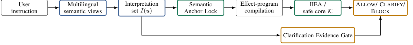
Fig. 1. Evaluated semantic-to-effect authorization path. The present paper evaluates the path through the final authorization decision; complete provider-side execution mediation remains future work.
